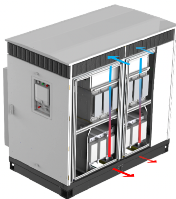
Heat dissipation cavity: Speed controlled fans for cooling
